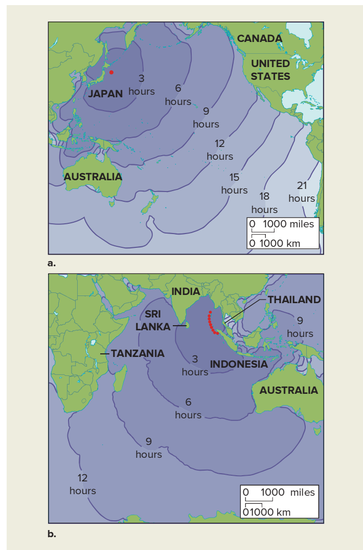
Figure 1.1 Travel times for recent tsunamis. a. Time taken for 2011 tsunami to travel to locations along the margins of the Pacific Ocean. b. Time taken for 2004 tsunami to travel to locations along the margins of the Indian Ocean.
