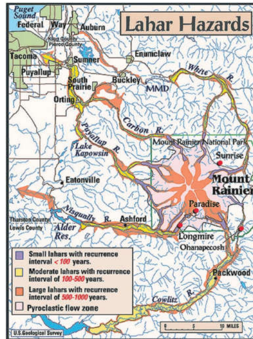
Figure 6.33 Lahar hazards associated with Mount Rainier, Washington. USGS
