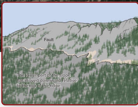
Figure 5.5 Signs of movement on a fault. Movement on a 44-kilometer-long (27-mile-long) fault caused the Hebgen earthquake in Montana in 1959. a. The fault broke the surface near a ranch (background). b. The fault can be followed for several kilometers along the south flank of Kirkwood Ridge in the center of the image. 5.5a: USGS, 5.5b: USGS
